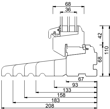
SILL PROJECTION OPTIONS
