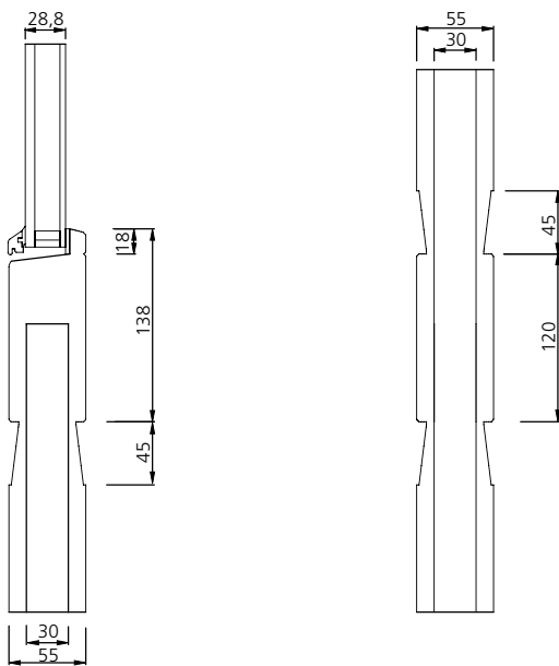
MID-RAIL
