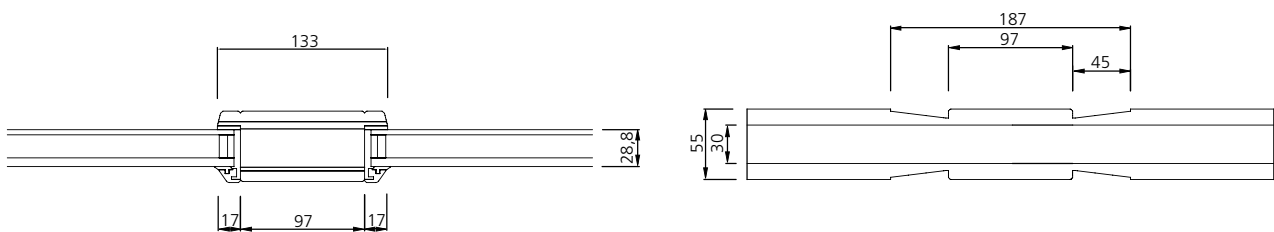
MULLION
