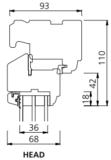
HEAD
