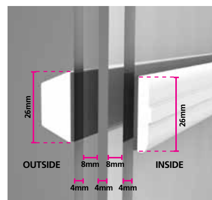
Simulated bars triple glazed
