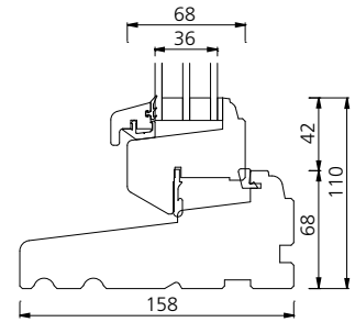
SILL
